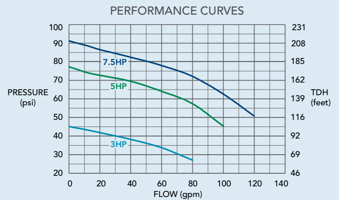
Pump HP selection chart
