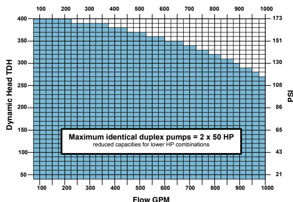
Pump HP selection chart
