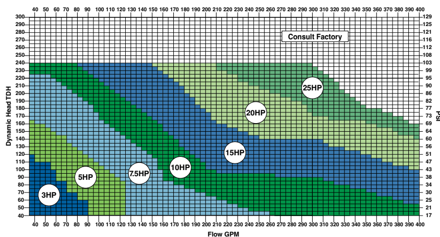
Pump HP selection chart
